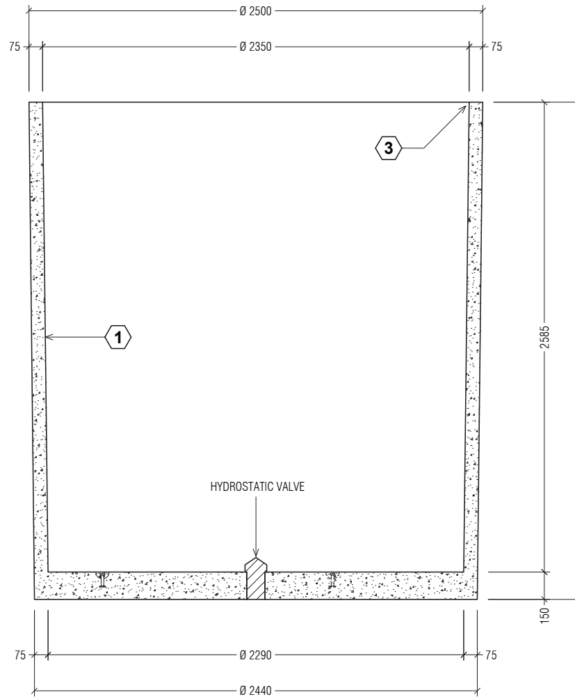
SECTION A-A (TANK)
