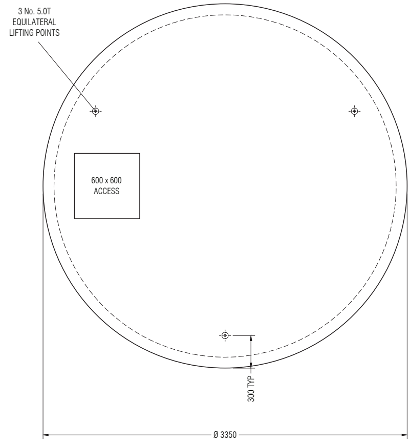
PLAN VIEW
