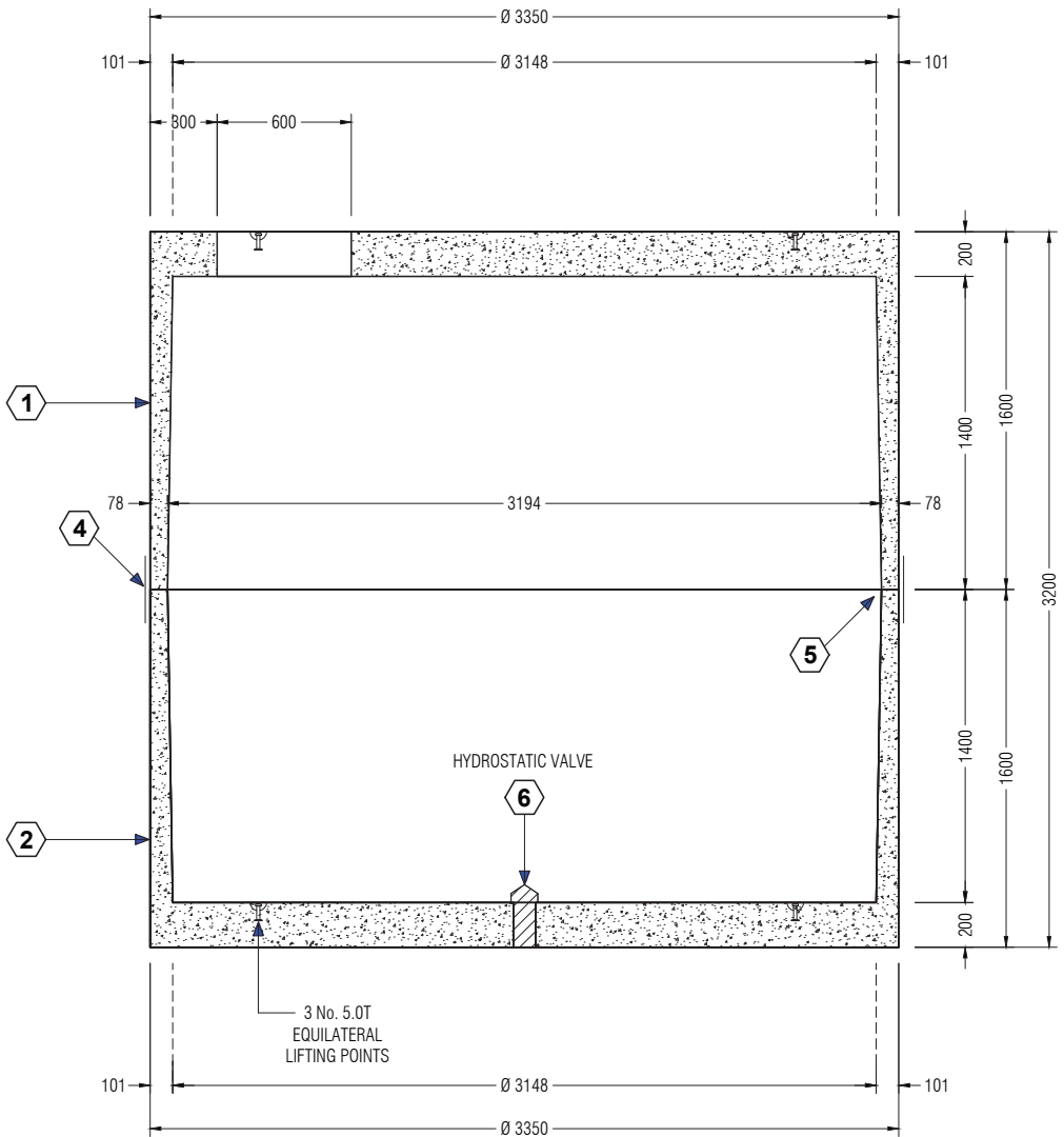
SECTION OF TANK
