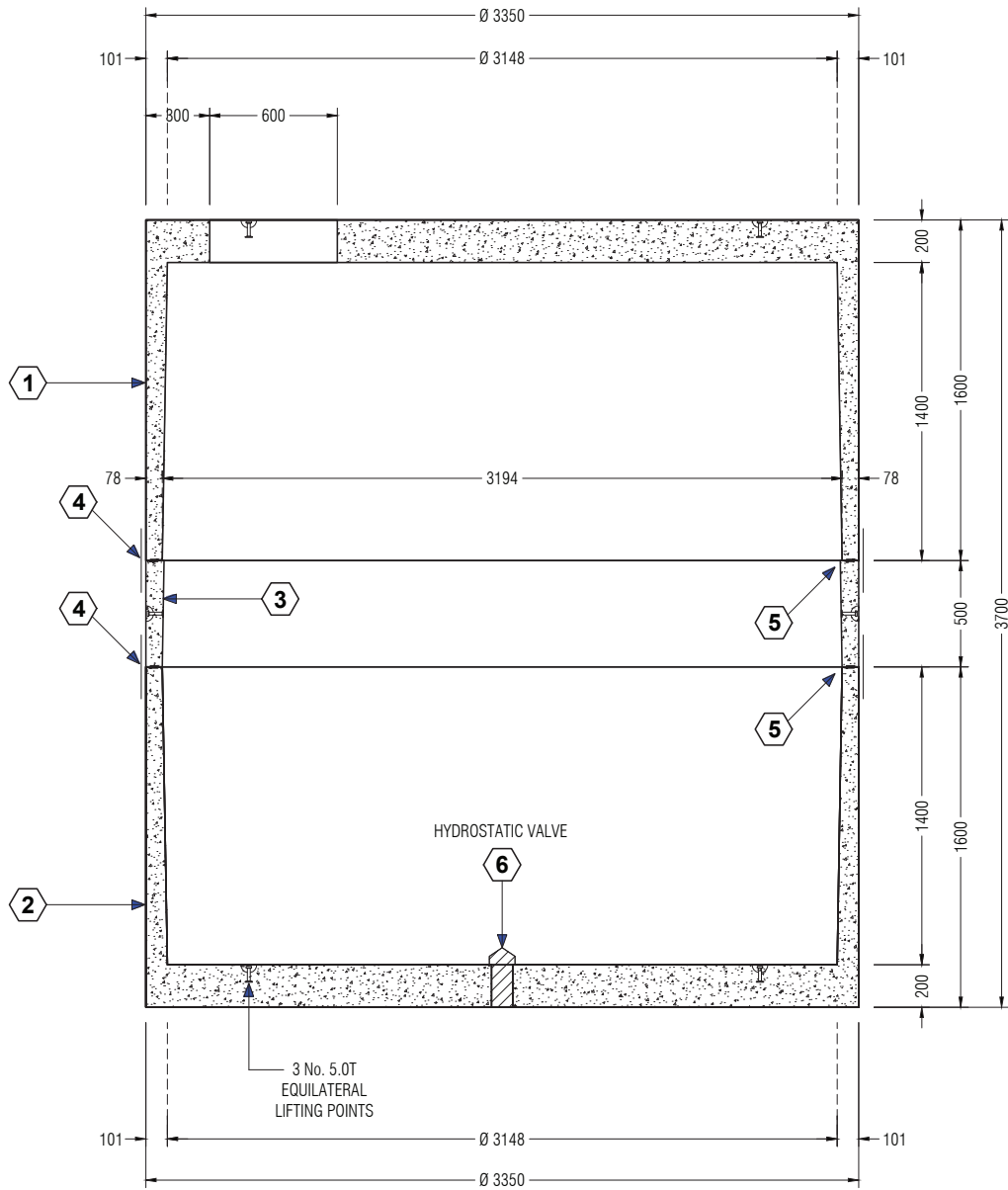
SECTION OF TANK
