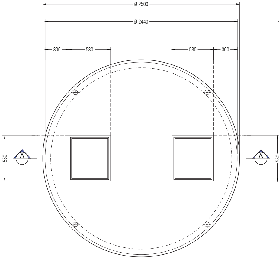
PLAN VIEW
