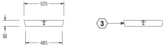
COVER DETAIL
