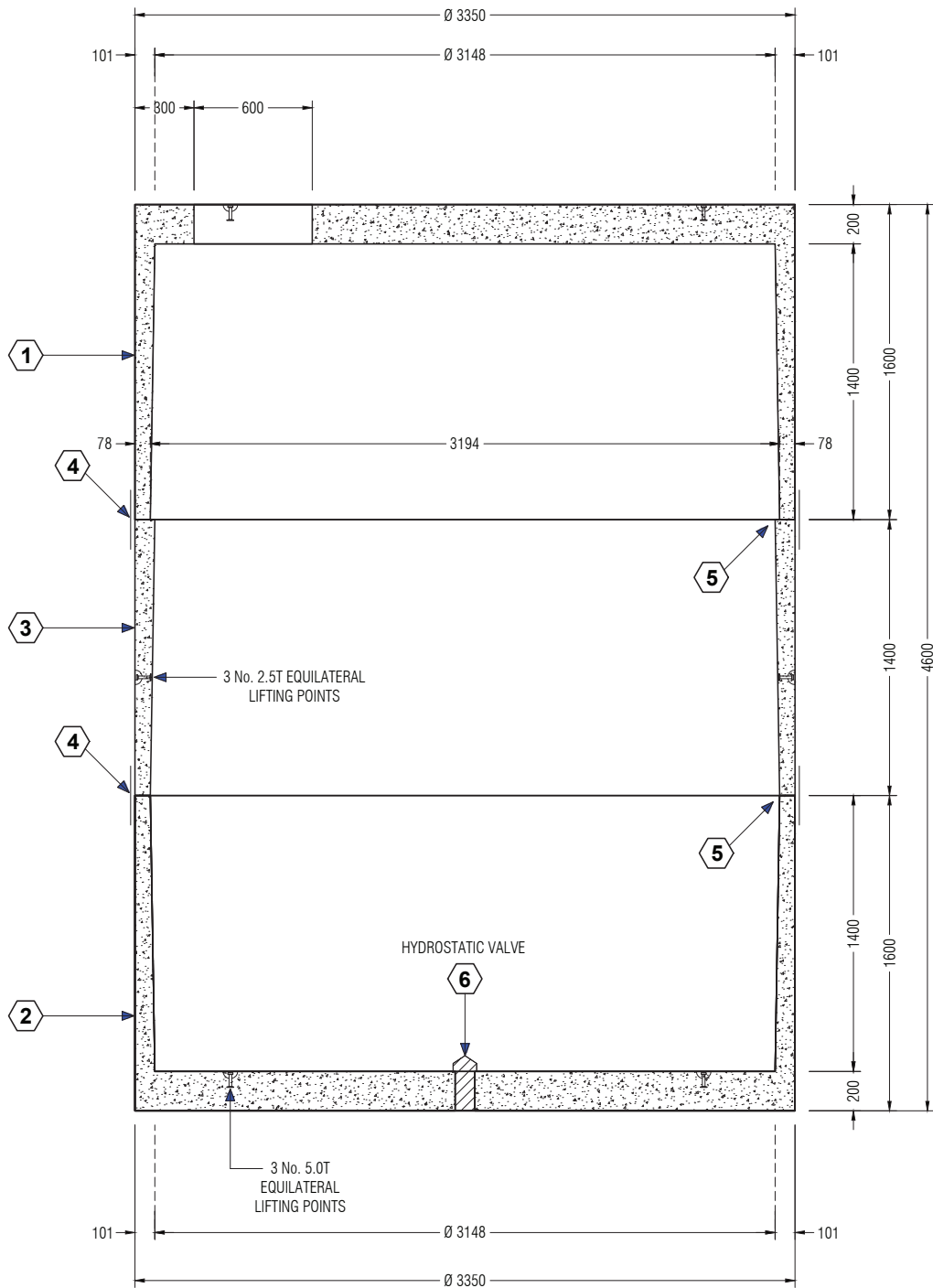
SECTION OF TANK
