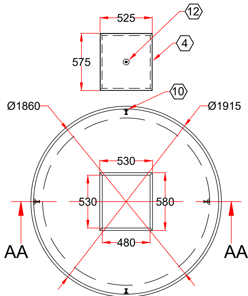
PLAN VIEW
